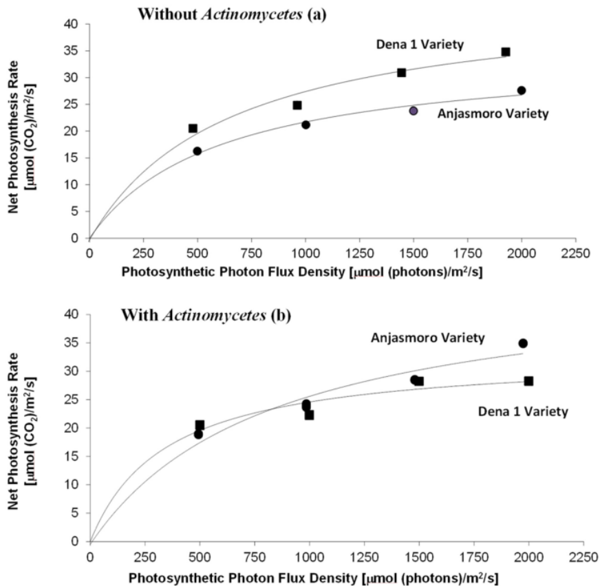
Fig. 1. Photosynthetic light response curve of Dena-1 and Anjasmoro variety under normal condition (a), and under Actinomyces spp. treatment (b)
